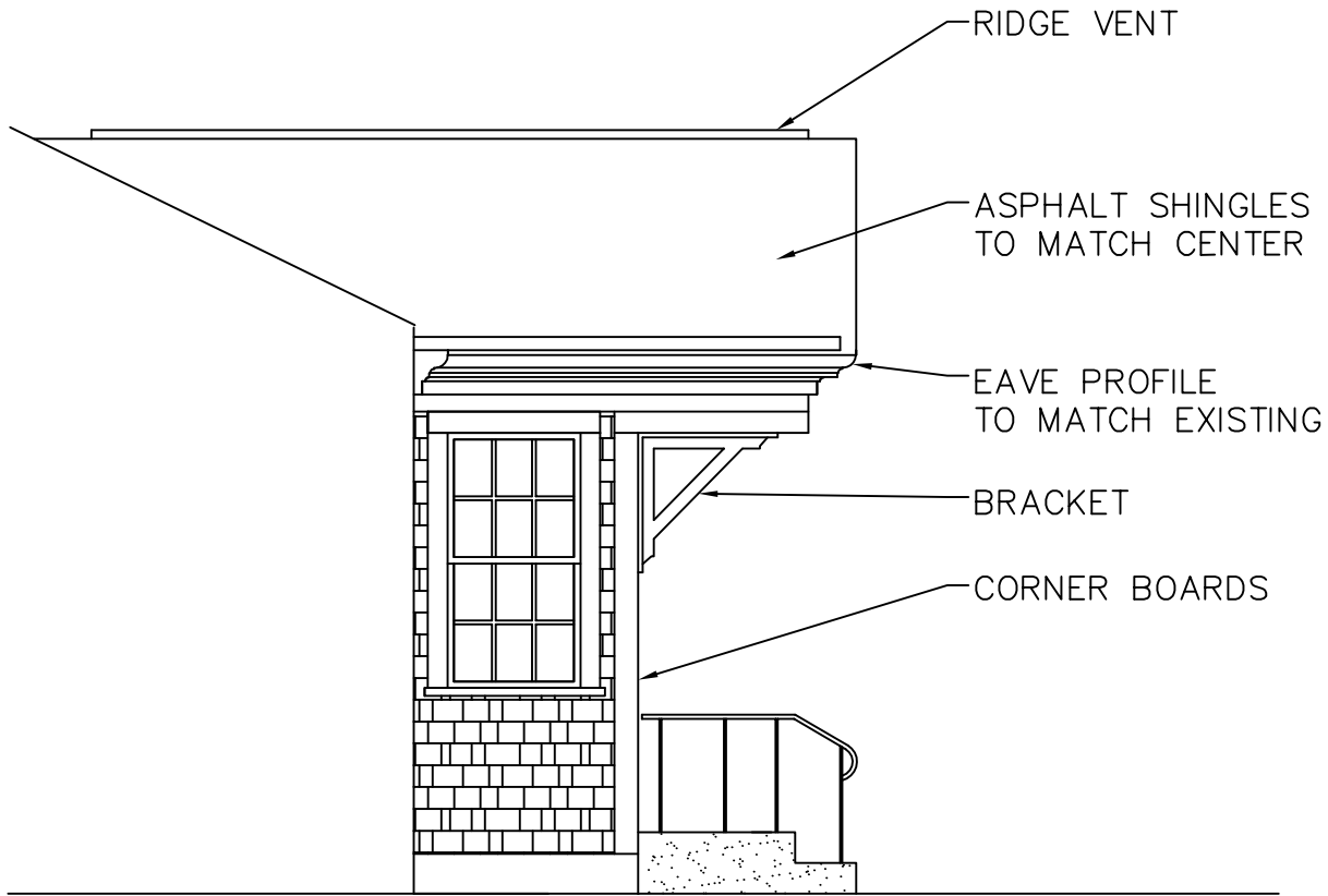
8 SIDE ELEVATION (BOTH SIDE TYPICAL)
